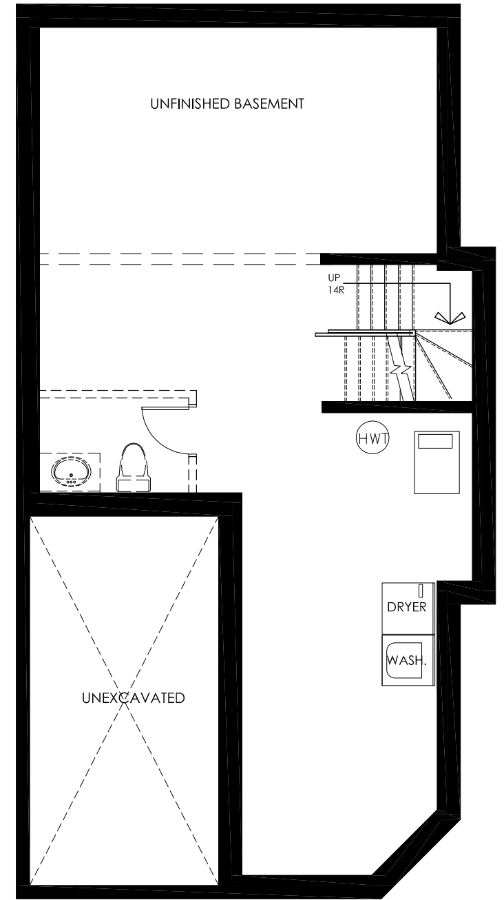
BASEMENT PLAN: 801 SQ. FT.
