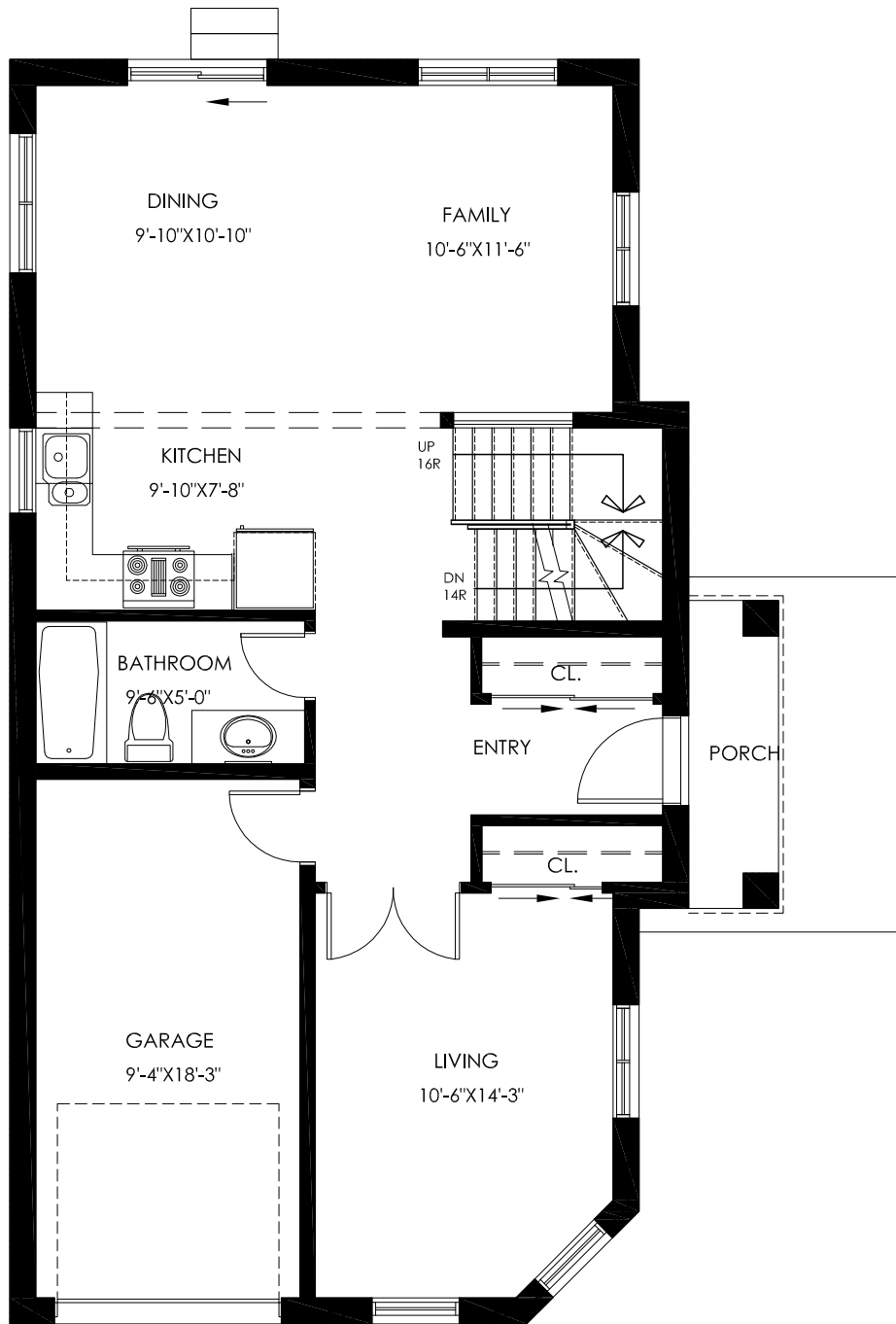
MAIN FLOOR PLAN: 816 SQ. FT.
