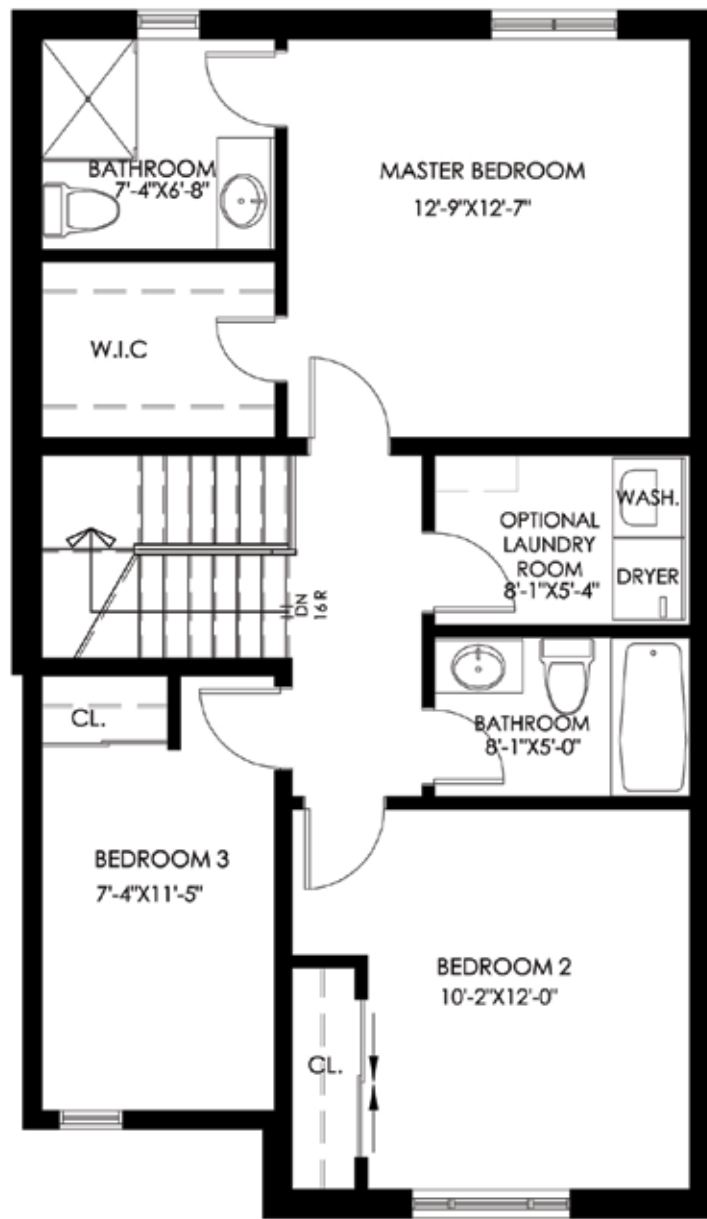
SECOND FLOOR PLAN: 835 SQ. FT.
