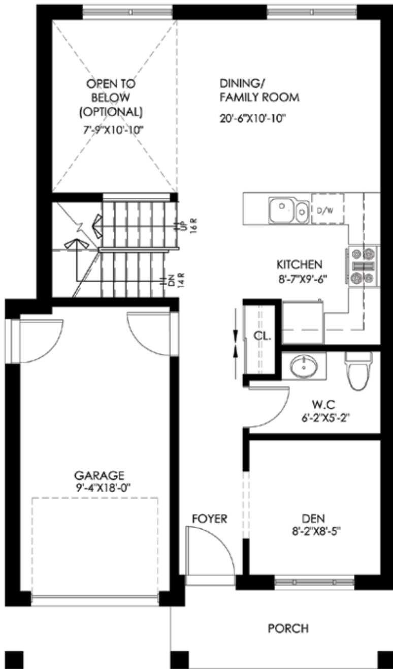
MAIN FLOOR PLAN: 665 SQ.FT.
