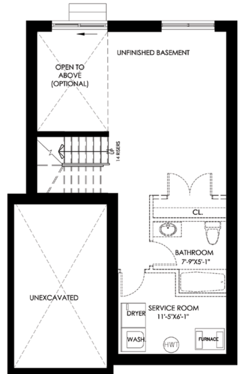
BASEMENT PLAN: 666 SQ. FT.
