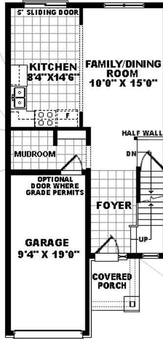
TH-4/TH-4END GROUND FLOOR PLAN
