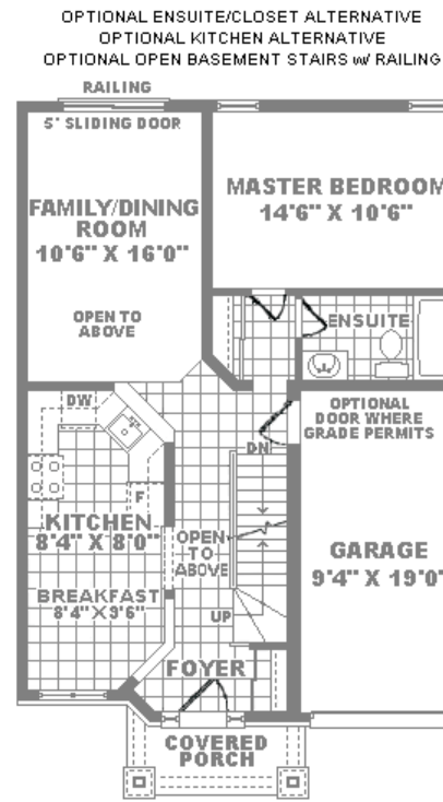
TH-3/TH-3 END GROUND FLOOR PLAN
