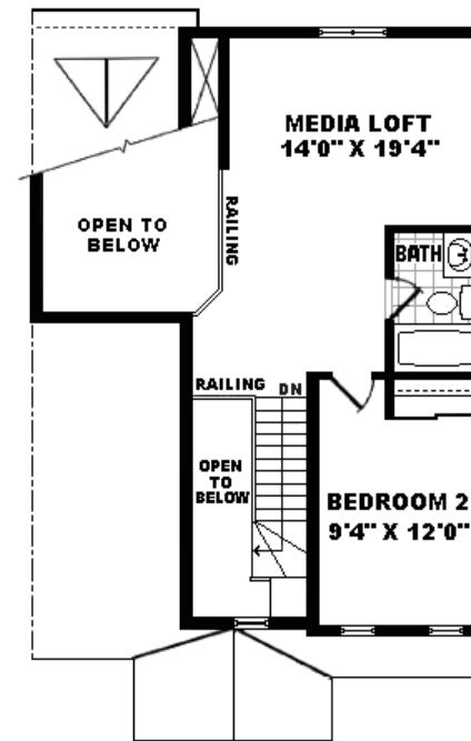
TH-3/TH-3 END LOFT FLOOR PLAN
