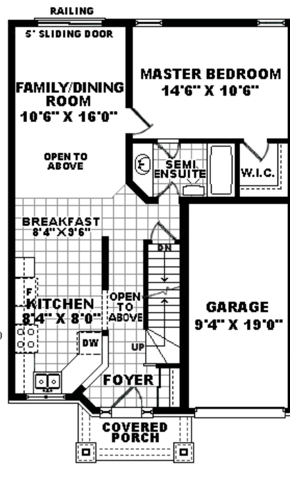
TH-3/TH-3 END GROUND FLOOR PLAN
