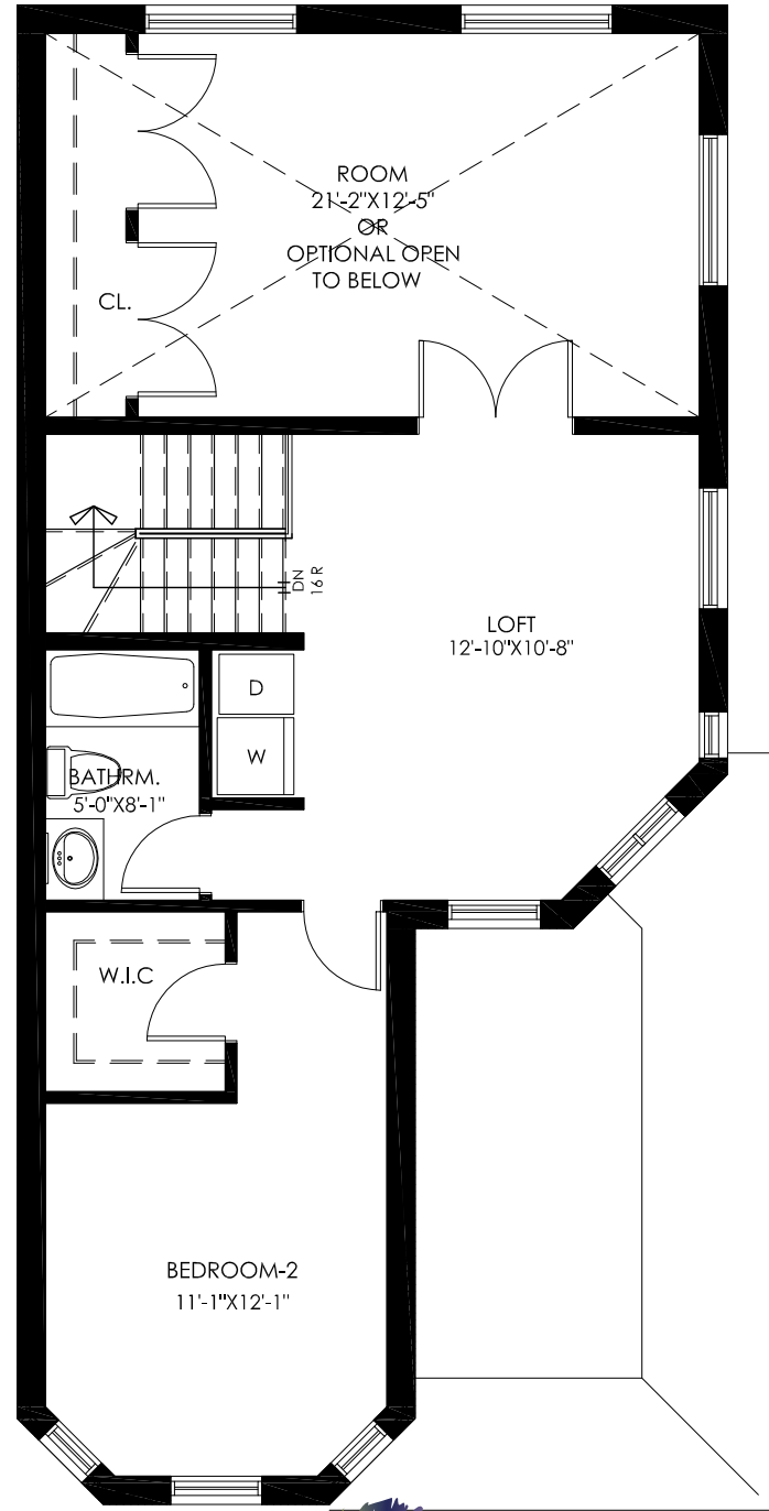
SECOND FLOOR PLAN: 888 SQ. FT.
