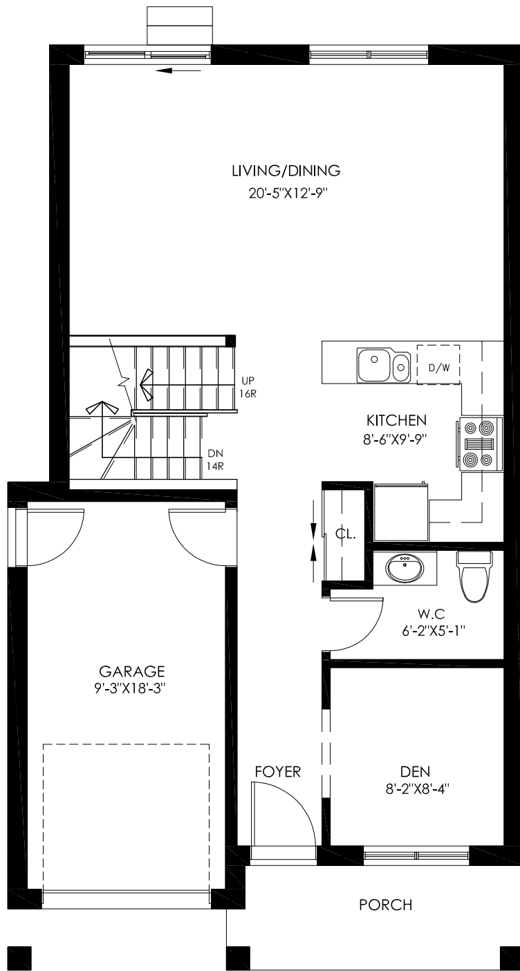
MAIN FLOOR PLAN: 720 SQ. FT.
