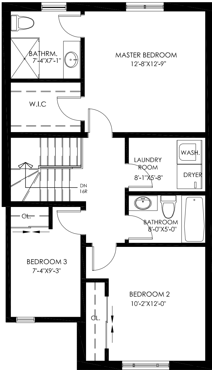
SECOND FLOOR PLAN: 795 SQ. FT.
