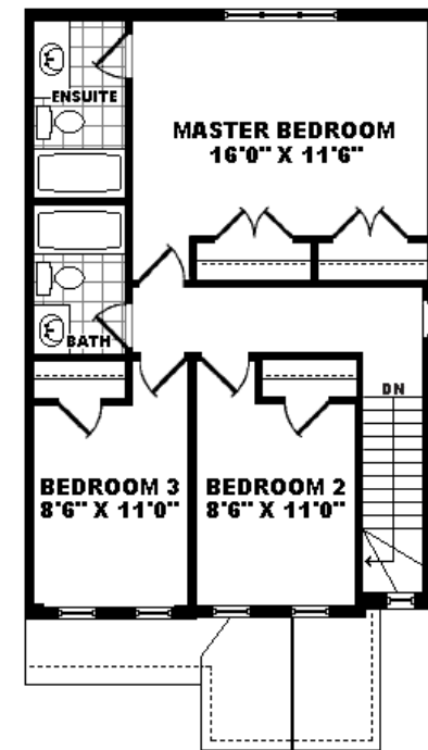
TH-7 END SECOND FLOOR PLAN
