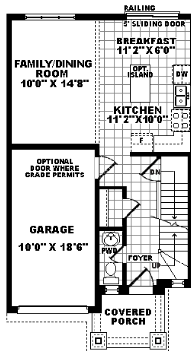
TH-7 END GROUND FLOOR PLAN
