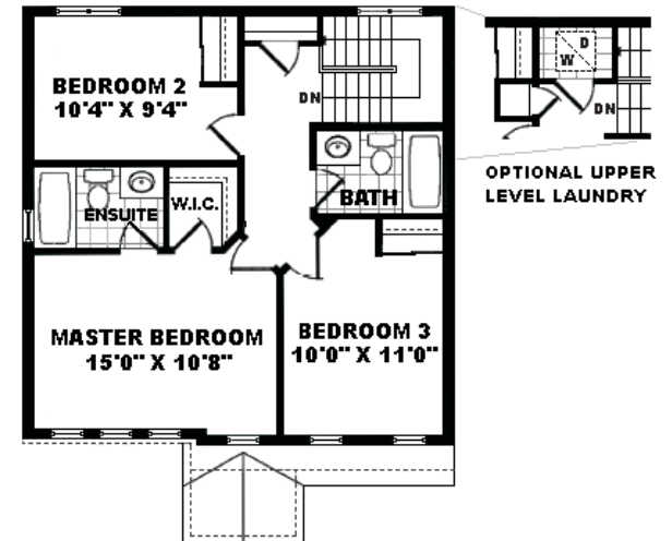
TH-6/TH-6 END SECOND FLOOR PLAN
