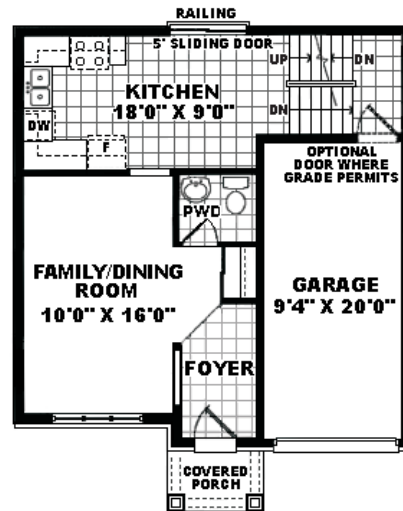
TH-6/TH-6 END GROUND FLOOR PLAN
